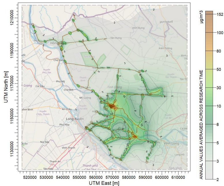
Figure 9. Annual average of TSP dispersion from transportation from 2021-2023
