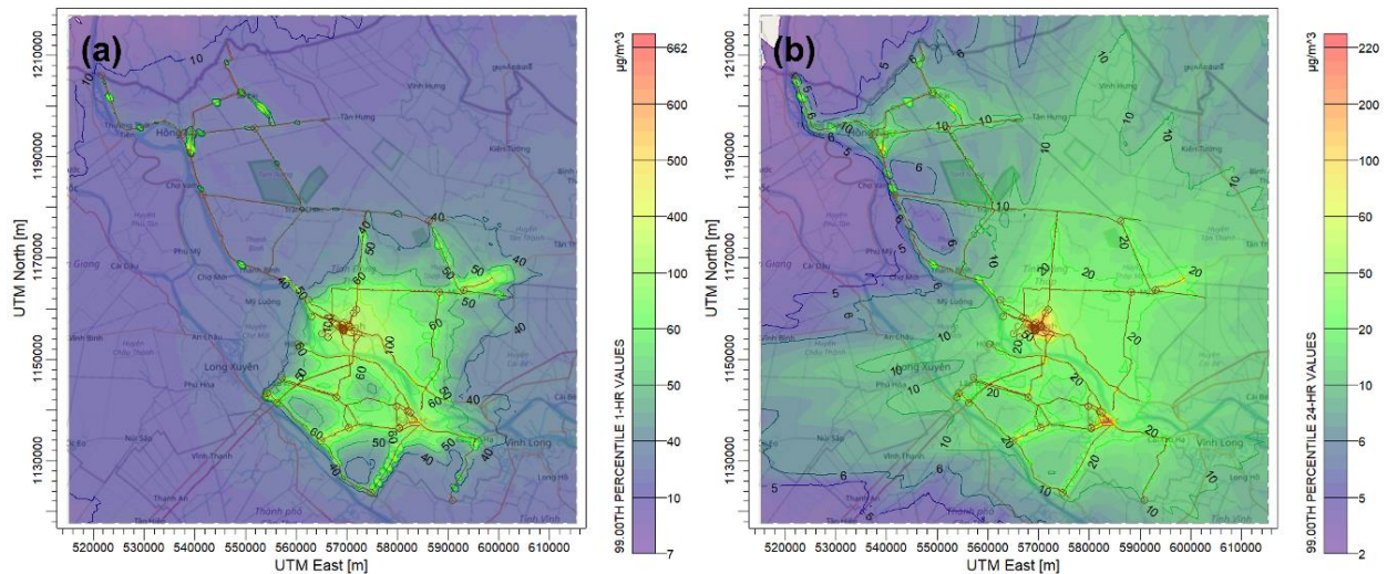
Figure 7. The 99 th percentile TSP dispersion events from transportation sources: (a) 1-hour average and (b) 24-hour average.
